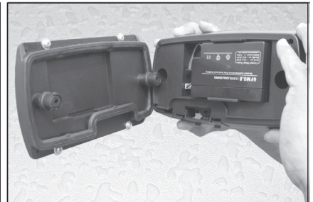
D. Reassemble Mounting Base and Electronics Console by Pushing the Two Pieces Together Firmly.
